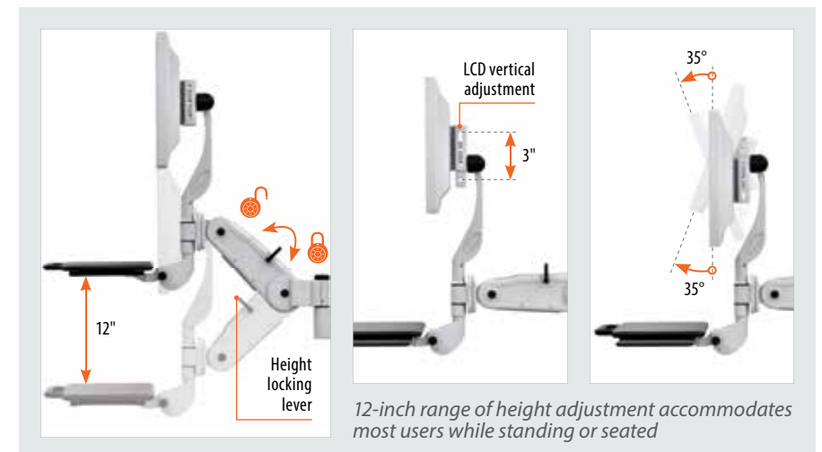
A. Pneumatically height-adjustable arm AFC7808 on 18-inch wall track
