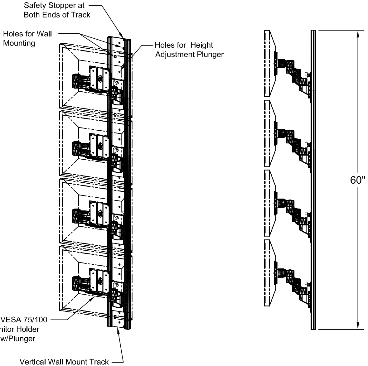
ISOMETRIC VIEW
