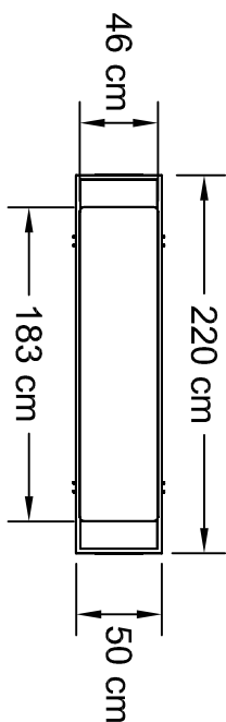
TOP VIEW of Center Console Scale: 1/4" = 1'-0"
